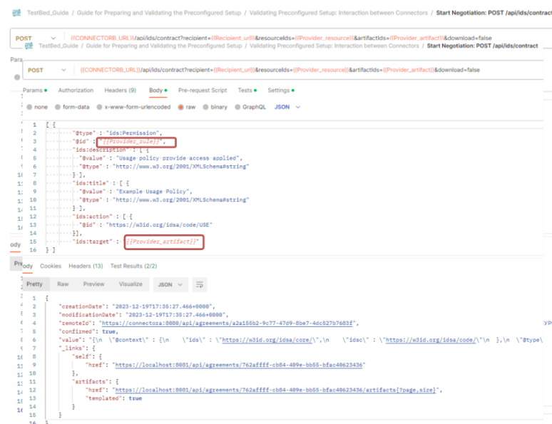
Figure 13. Dataspace API for negotiation between OEM and supplier. (“Provider_rule” and “Provider_artifact” are marked with red box)
