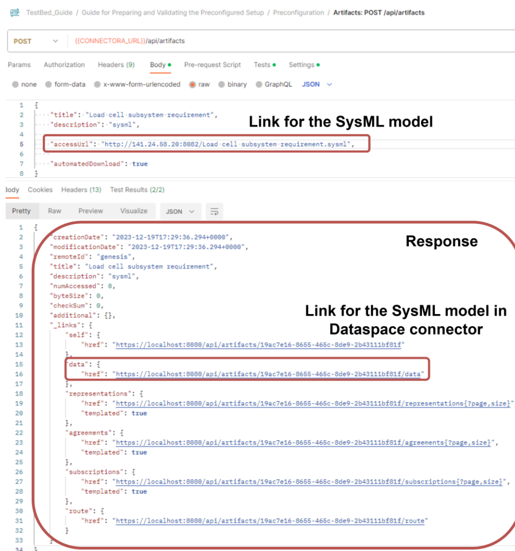
Figure 12. Dataspace API for data upload in Postman.
