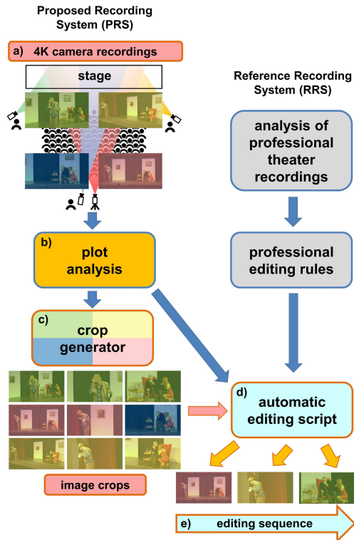
FIGURE 4. Schematic structure of the Proposed Recording System (PRS).
