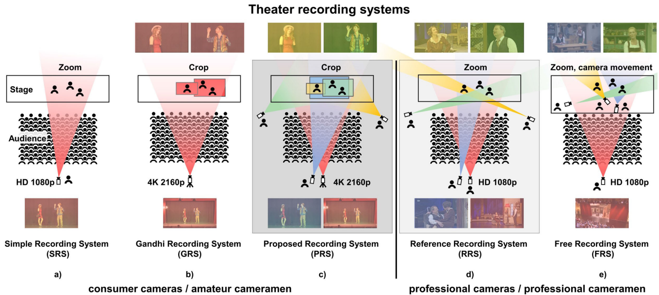
FIGURE 3. Theater recording systems. Amateur recording systems on the left side: a) Simple (without cuts), b) Gandhi cropping close-ups ([3]), c) Proposed Recording System with four cameras and cropping. Professional recording systems on the right side: d) Reference Recording System with four fixed-position cameras, e) Moving cameras on stage.
