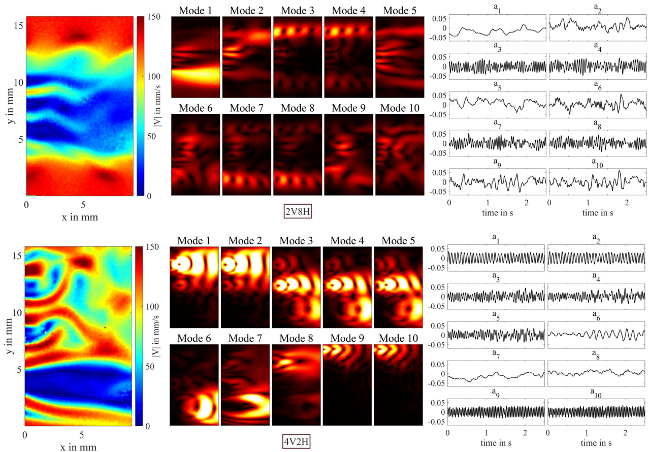
FIG. 8. The instantaneous absolute velocity field |V| (left), the spatial POD modes (center), and their corresponding time coefficients (right) for the 2V8H and 4V2H arrays at top and bottom, respectively.
