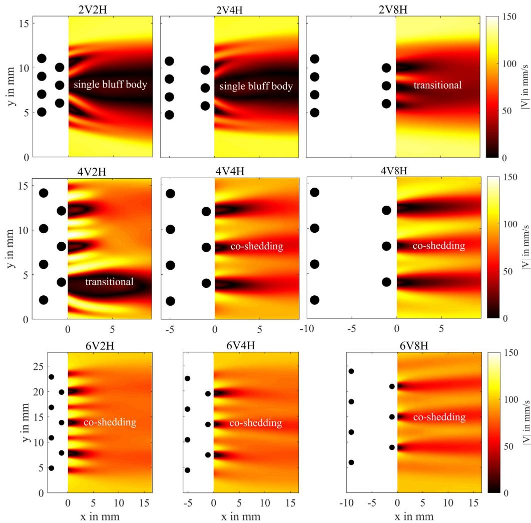
FIG. 3. Time-averaged absolute velocity ( |V| ) field behind the arrays. The free stream velocity is V_\infty = 133 mm/s.
