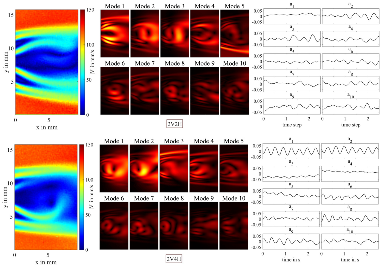
FIG. 7. The instantaneous absolute velocity field |V| (left), the spatial POD modes (center), and their corresponding time coefficients (right) for the 2V2H and 2V4H arrays at top and bottom, respectively.
