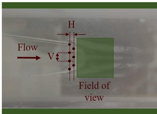
FIG. 1. Photograph of the field of view for the PIV measurements and the arrangement of the cylinders in the flow. In total, there are nine different sets of cylinders, with V = [2, 4, 6] mm and H = [2, 4, 8] mm.
