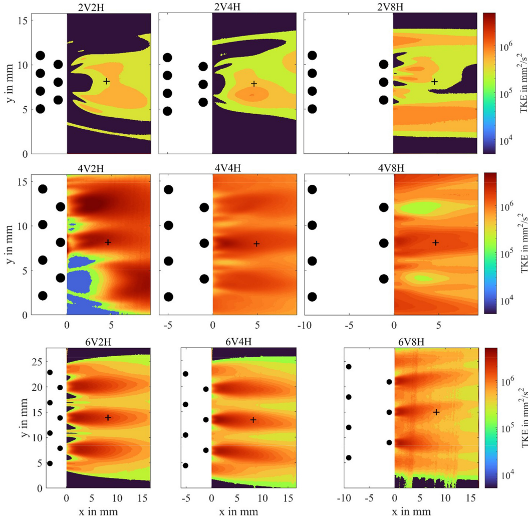
FIG. 4. Total kinetic energy (TKE) distribution behind the arrays. The black crosses at the center of each TKE field represent the coordinates of the points, which were used to show the evolution of the mean horizontal velocity u over time in Fig. 2.
