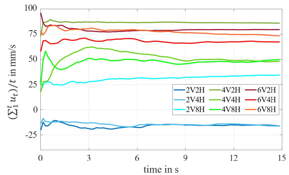
FIG. 2. The evolution of the mean value for the horizontal velocity u over time at the middle of the field of view for each array.
