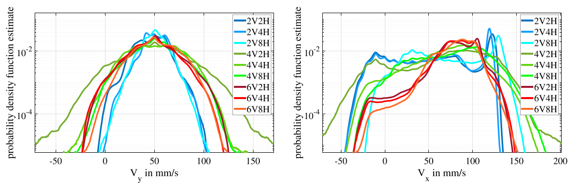
FIG. 5. Probability density function (PDF) of the vertical (left) and horizontal (right) velocity components for the arrays.
