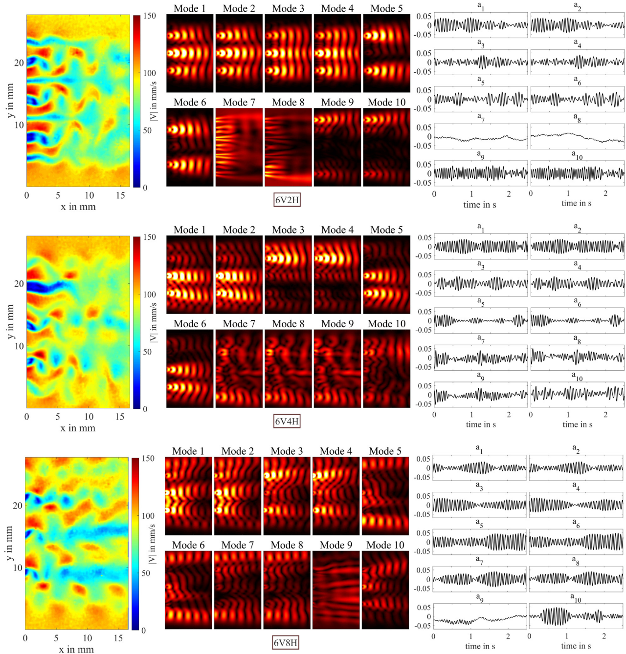
FIG. 10. The instantaneous absolute velocity field |V| (left), the spatial POD modes (center), and their corresponding time coefficients (right) for the 6V2H, 6V4H, and 6V8H arrays at top, middle, and bottom, respectively.
