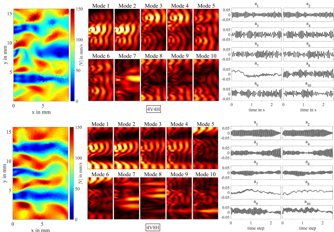
FIG. 9. The instantaneous absolute velocity field |V| (left), the spatial POD modes (center), and their corresponding time coefficients (right) for the 4V4H and 4V8H arrays at top and bottom, respectively.
