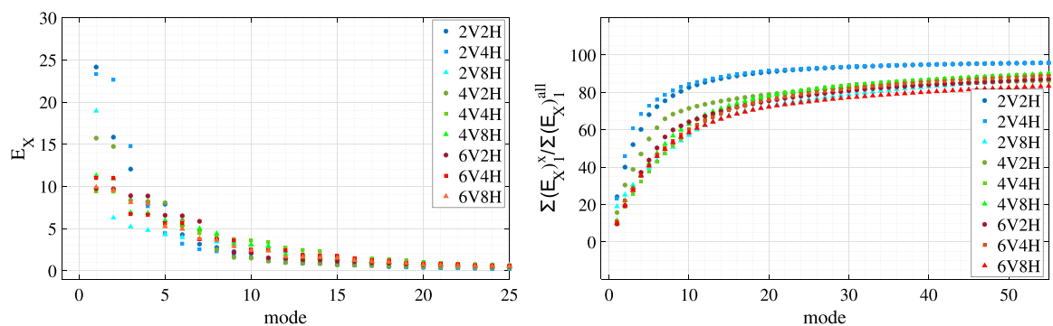
FIG. 6. Energy of POD modes for the arrays. Modal kinetic energy percentage (left) and sum of kinetic energy percentage (right).
