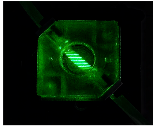
Fig. 8. Measurement chamber with inserted FEP-tube filled with water and illuminated by the multiple light sheets.
