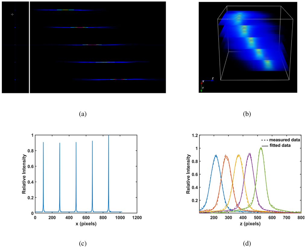
Fig. 7. (a) Display of the five focal spots in the x - z plane. (b) Cube of 6\text{ mm} \times 6\text{ mm} \times 6\text{ mm} showing the five light-sheets in 3D. (c) 1D Intensity distribution of the normalized intensity distribution in vertical direction ( x -axis). (d) The normalized Intensity distribution of measured data, each fitted with a Gaussian function in axial direction ( z -axis).
