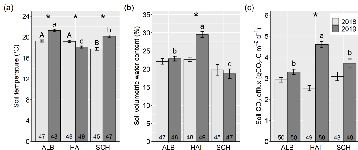
Figure 3.1 (a) Soil temperature at 5 cm, (b) soil volumetric water content at 10 cm soil depth and (c) soil respiration in 2018 (light grey) and 2019 (dark grey) for the three study regions; Schwäbische-Alb =ALB; Hainich-Dün =HAI and Schorfheide-Chorin =SCH. Bars show mean values and error bars show the standard error of the samples. Numbers at the base of the bars indicate the number of observations available in each study region and year. Asterisks indicate significant differences between the years for a given study region according to post-hoc tests. Upper (for 2018) and lower-case letters (for 2019) indicate differences among the three study regions in the two years.
