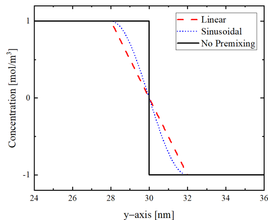
Figure 3. Possible mathematical concentration profile models of the intermixed zone at the bilayer interface and between the bilayers.
