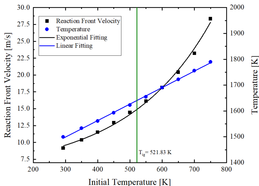
Figure 12. Influence of initial temperature of the reactive multilayer foil on the propagation reaction front velocity and temperature.
