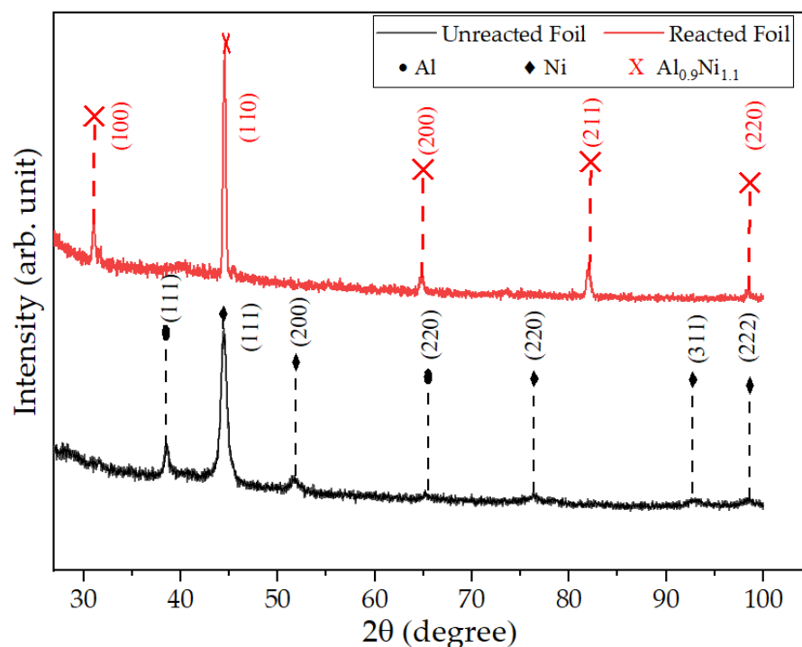
Figure 7. X-ray Diffraction analysis of free-standing Al/Ni multilayer foils before and after the self-propagating reaction.
