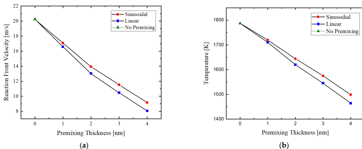
Figure 9. The effect of sinusoidal and linear premixing zone (explained in Section 2.2) on (a) the reaction front velocity and (b) the reaction temperature at the reaction front, where E_a = 107 \text{ kJ mol}^{-1} , D_0 = 2.18 \times 10^{-5} \text{ m}^2\text{s}^{-1} and heat of reaction is calculated by Equation (6). (Lines are drawn to guide the eyes).
