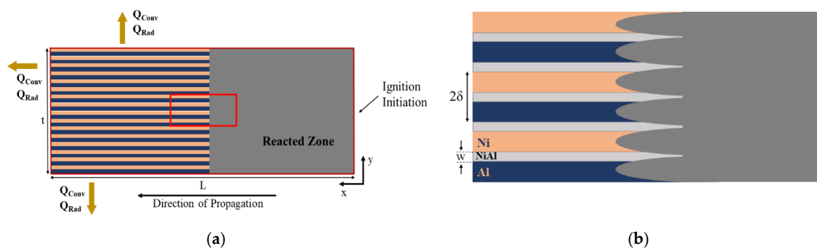
Figure 2. (a) Schematic of the implemented model. Q_{conv} and Q_{rad} are convective heat loss and radiative heat loss (b) enlarged view of the selected red area in (a), where w is the intermixing thickness of the multilayers and 2\delta is the bilayer thickness.
