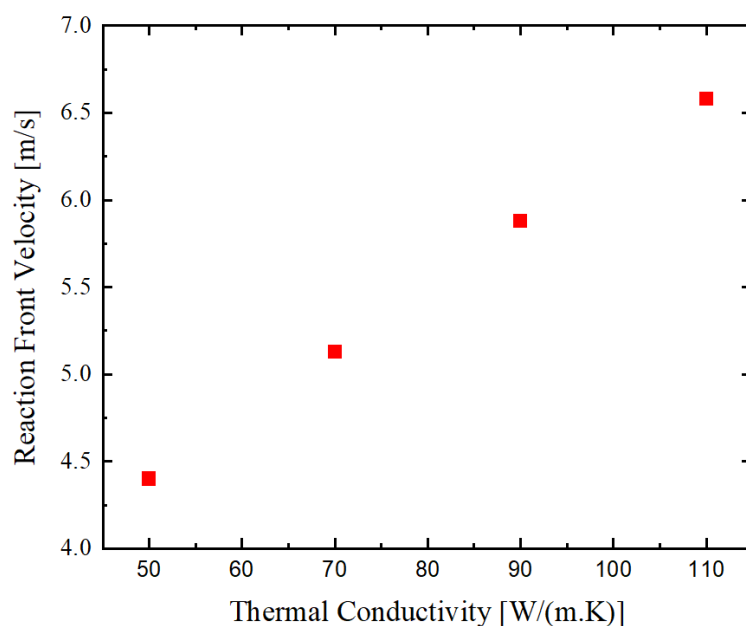
Figure 10. Influence of thermal conductivity of the final reaction product on the self-propagating reaction front velocity.
