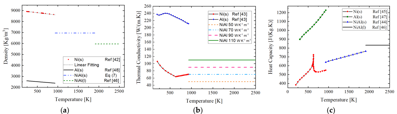
Figure 5. (a) Temperature dependent density of Al and Ni in solid-state; dotted line shows the linear fitting of data extracted from [42]. For temperatures greater than 933 K, the density of NiAl in the solid and liquid state is plotted. (b) Temperature dependent thermal conductivity of Nickel and Aluminum in solid-state taken from [43]. It is combined with different values of thermal conductivity of product (NiAl). (c) Temperature dependent heat capacity of Ni, Al in solid-state, and NiAl in both solid and liquid state extracted from [44–47].
