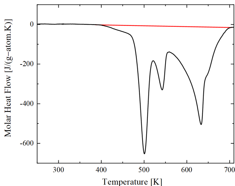
Figure 4. Molar heat flow curve of free-standing thin films for an equiatomic Al/Ni multilayer with a 50 nm bilayer periodicity measured with a constant heating rate of 0.333 K s ^{-1} . The red line displays the upper limit for the area of integration that was used for the determination of the total enthalpy release.
