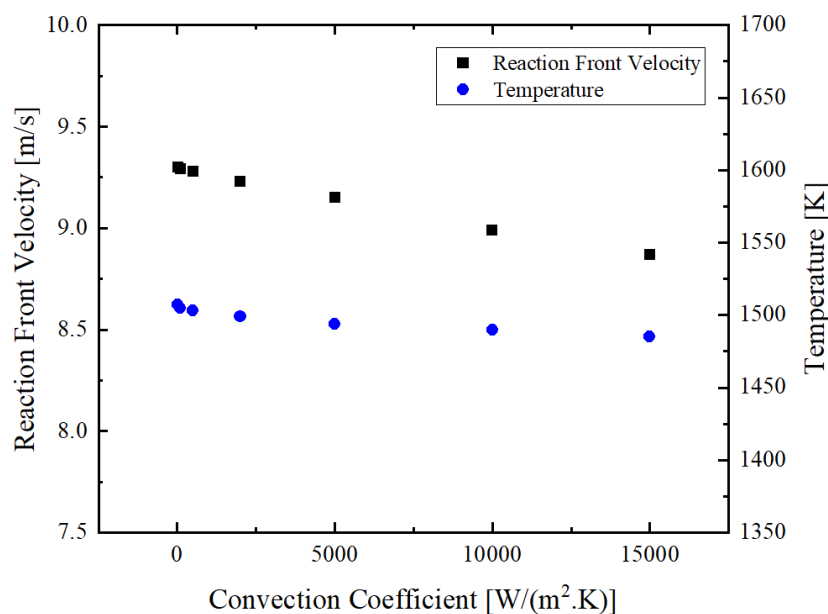
Figure 11. Effect of changing the ambient condition (convective coefficient) on the reaction front velocity and the temperature at the reaction front.
