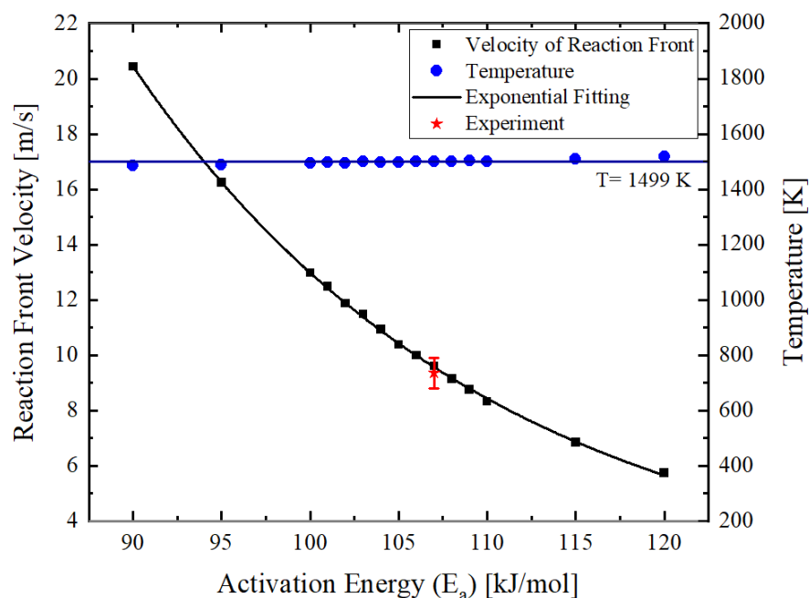
Figure 8. Effect of the activation energy of diffusion on the reaction front velocity and the reaction temperature at the reaction front. The width of the intermixing zone was set to 4 nm.
