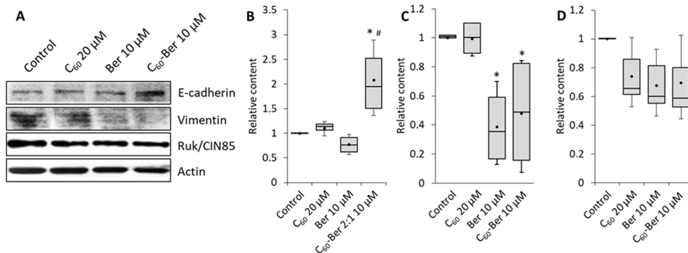
Figure 3. C_{60} -Ber nanocomplex modulates the content of EMT molecular markers in LLC cells: (A)—representative results of Western-blot analysis; (B–D)—quantitative analysis of E-cadherin, vimentin, and Ruk/CIN85 content, respectively. Box-plot legend: box represents second and third quartiles; whiskers—minimal and maximal values; dot—mean value. * p < 0.05 compared to control; # p < 0.05 compared to free Ber.
