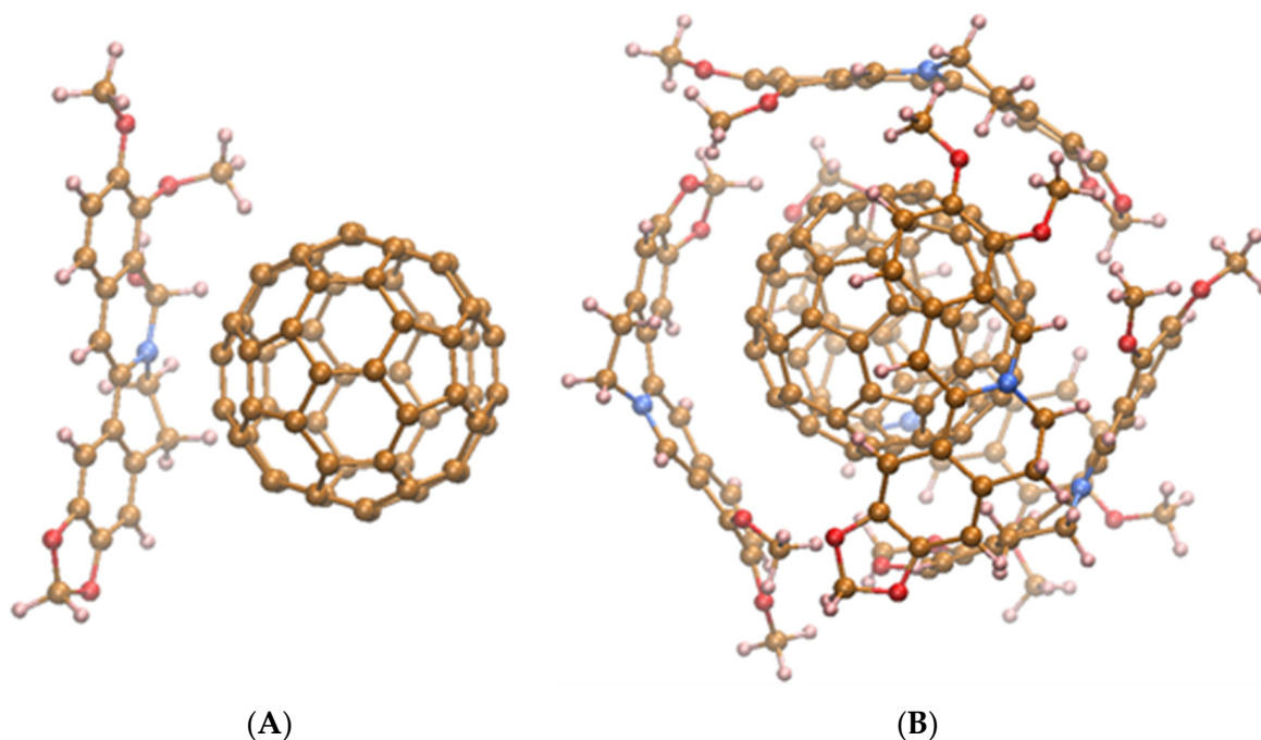
Figure 1. The energy-minimized structure of nanocomplexes formed at C_{60} binding with one (A) or five (B) Ber molecules.
