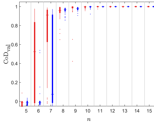
Figure 2: Boxplot of the \text{CoD}_{\text{val}} for the distance-based LOO error method (left) and LHS method (right) depending on n for the approximation of x \sin x
