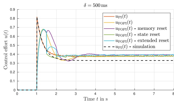
Fig. 7. Experimental control effort.
