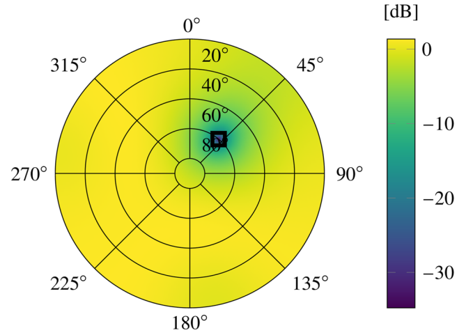
(A) unambiguous for \delta_{\text{ura}} = \frac{\lambda}{2}
