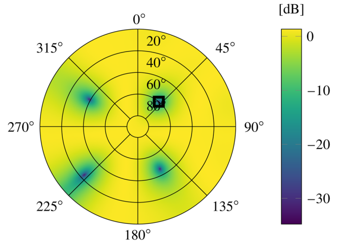
(B) rank-one ambiguity for \delta_{\text{ura}} = \lambda
