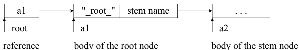
Figure 5 : Root and stem nodes of an R - tree
