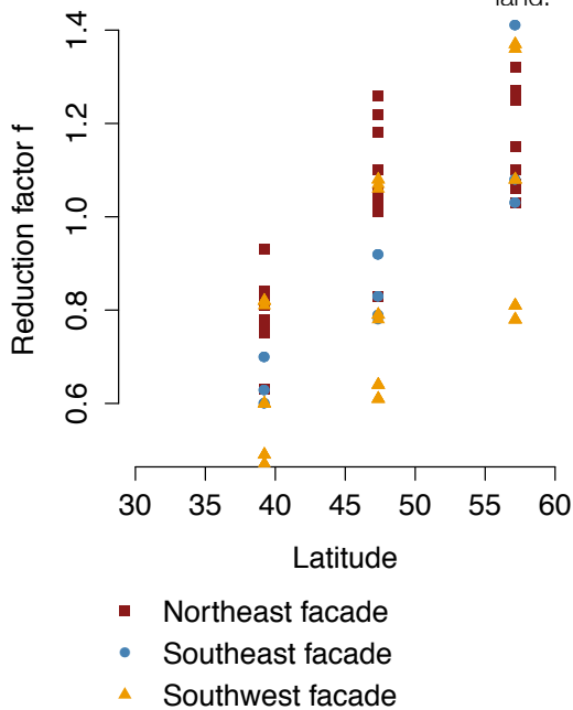
Calculated reduction factors compared to latitude of the specific location.
