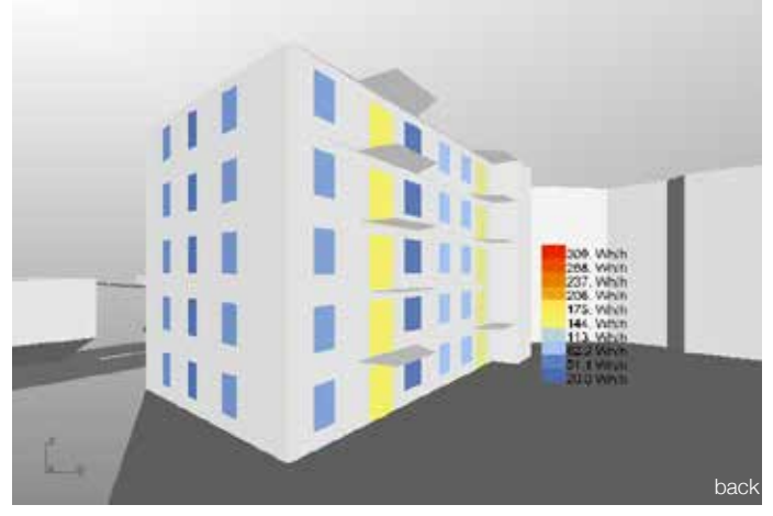
Window dimensions and total radiation entering the windows of the adapted Situation for Zurich.
