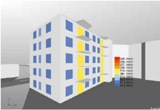
Window dimensions and total radiation entering the windows of the initial Situation for Zurich.
