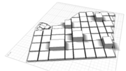
Fig. 29 Shadow Analysis in Summer (Vertical Plan 3)
