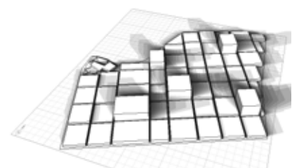
Fig. 32 Shadow Analysis in Winter (Vertical Plan 3)
