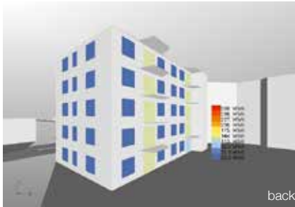
Window dimensions and total radiation entering the windows of the initial Situation for northern Scotland.
