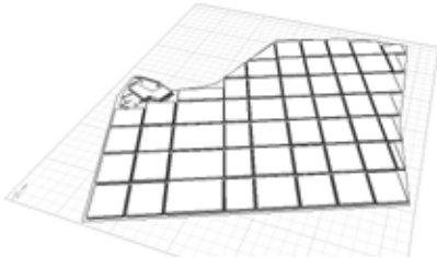
Fig. 27 Shadow Analysis in Summer (Vertical Plan 1)
