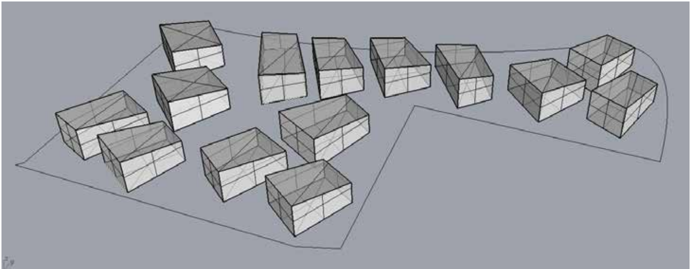
Final Volumes of the Reorganized Hunziker Areal according to the Solar Envelope Concept
