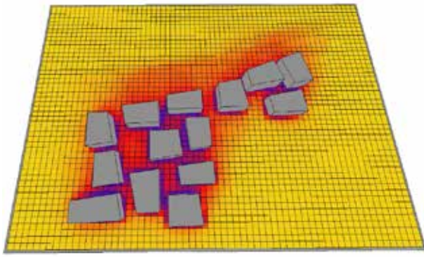
Winter Solstice Insolation Analysis as-planned
