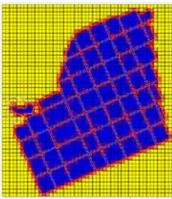
Fig. 33 Solar Radiation Analysis in Summer (Vertical Plan 1)
