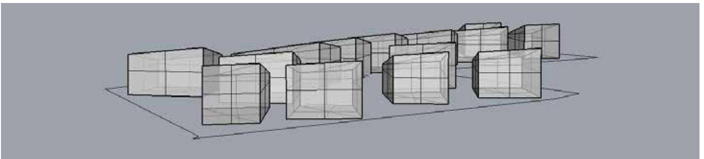
Viewed from Winter Solstice Sun Position at 15.00
