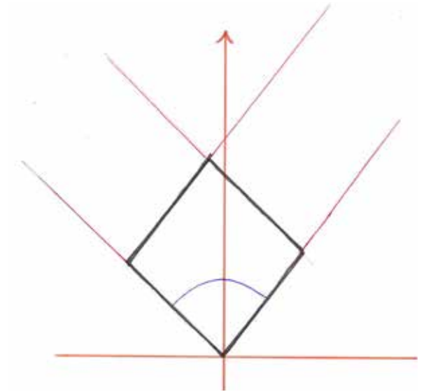
Optimal Orientation of Buildings for Reduced Shadow Area
