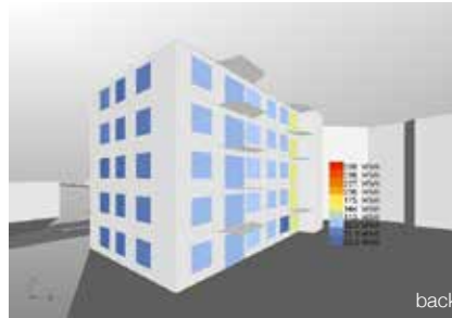
Window dimensions and total radiation entering the windows of the adapted Situation for northern Scotland.
