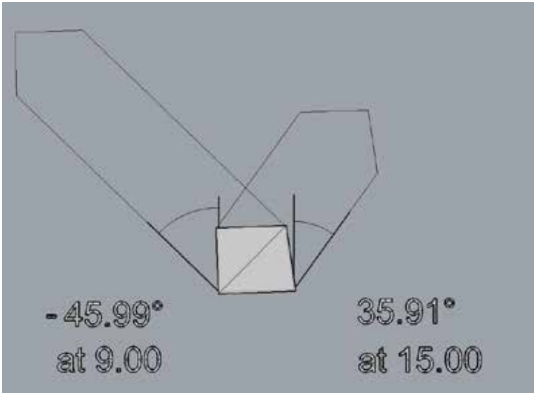
Winter Solstice Shadow Projections on Building I
