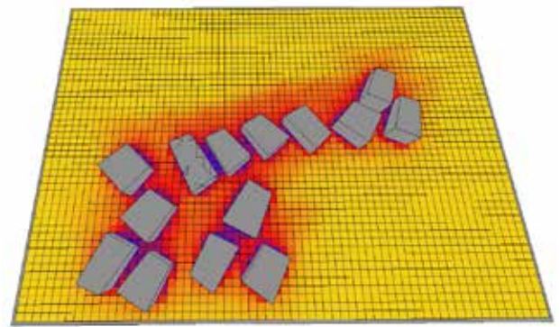
Winter Solstice Insolation Analysis as Reorganized
