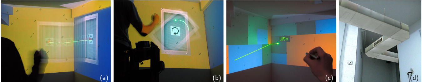
Figure 1: Basic object manipulation techniques such as translation (a) and rotation (b) are illustrated in long exposure photographs. Augmentation can be projector-based (a-c) or via video-see-through (d). These application examples show basic augmentations of building structures (a,b,d), distance measurements (c) and material-color simulations (c).
