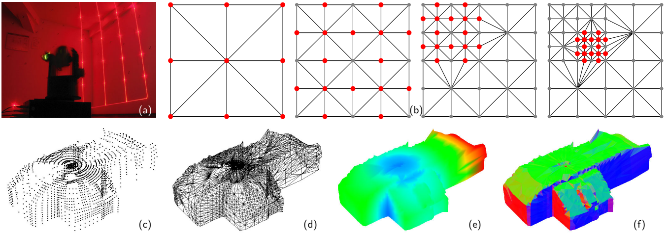
Figure 5: Sampling surface geometry: long exposure recording of the sampling process of the PTZ camera (a), adaptive multi-resolution sampling examples with vertex connectivity for the first four sample levels (b), sampled point cloud of entire room (c), triangulated surface geometry (d), depth map (e) and normal map (f).
