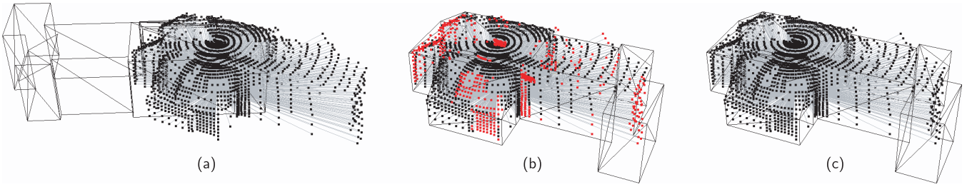
Figure 7: Unregistered sampled points and reference model (a), first registration step with identified outliers marked in red (b) and a mean registration error of 3.6 cm (in world coordinates), and final solution with minimal error of less than 1cm (c).
