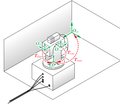
Figure 6: Transformations between local and global coordinate systems of the PTZ camera.
