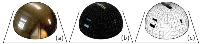
Figure 9: Spherical environment texture: captured under normal exposure (a) and under short exposure (b). Binary mask of invalid areas unsuited for laser pointer tracking (c).
