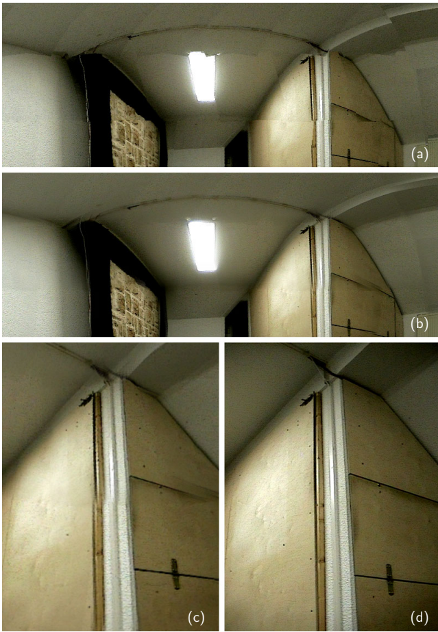
Figure 8: Sampling surface reflectance: 81 partially overlapping normal exposure images capture the surface reflectance at all possible angles (a), blended images that lead to a single consistent environment map (b), a close-up on a fraction of the blended environment map (c), and a photograph from the same view (d). Slight misregistrations are due to small calibration errors.
