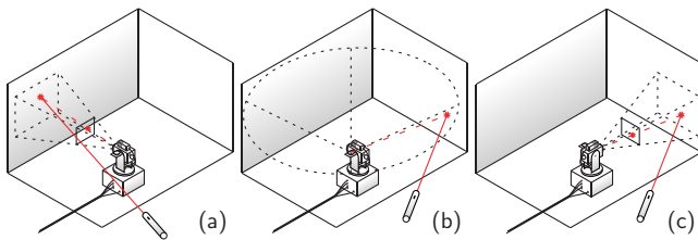
Figure 10: Tracking a laser spot in a 3D environment: If visible in the detail camera (a), the position of the laser spot can be estimated. If the spot is lost (b), the context camera delivers information for re-aligning the detail camera (c).
