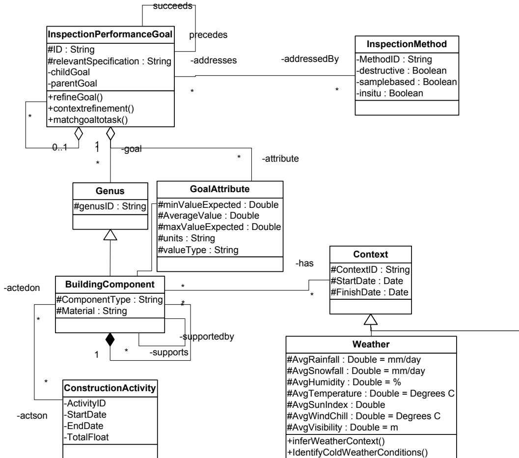
Figure 3: Inspection performance goals can be refined into sub-goals by reasoning with parent and child attributes and information about the context in which inspection will be performed.
