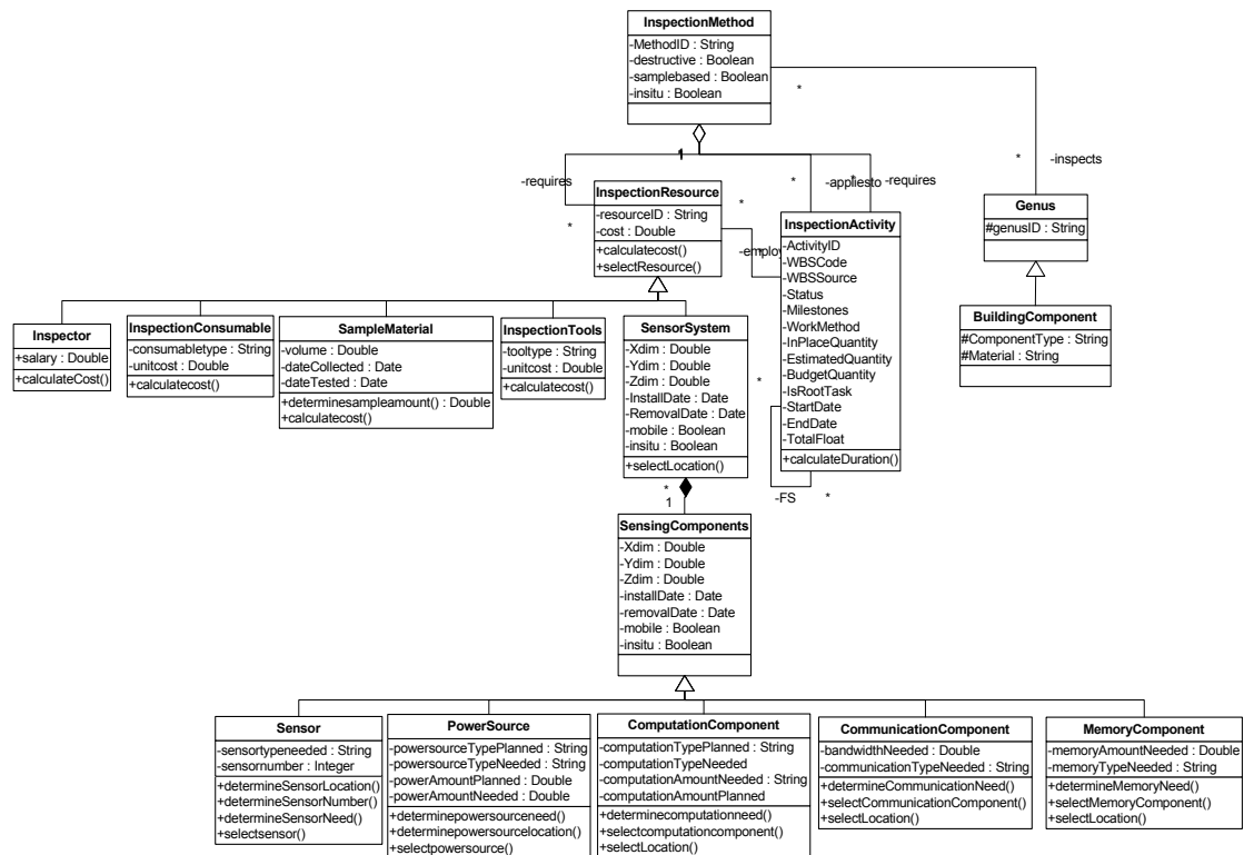
Figure 6: Methods can reason with inspection method knowledge and with features of the object to be inspected in order to calculate cost, duration, and location of inspection resources and activities.
