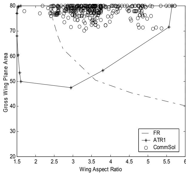
Figure 8 Common Region identified using high information gain variables 5,7 and 8 and all the solutions for K=3
