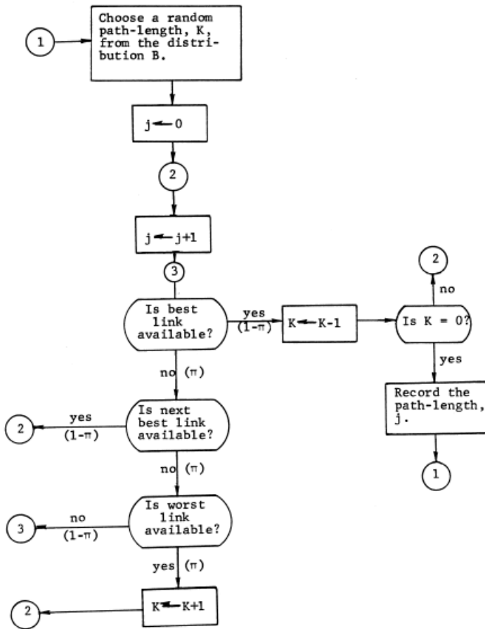
Fig. 2 Flowchart of Model A
