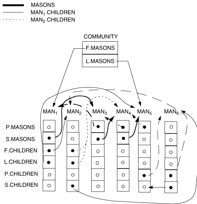
Figure 4-6. Set Relationships
