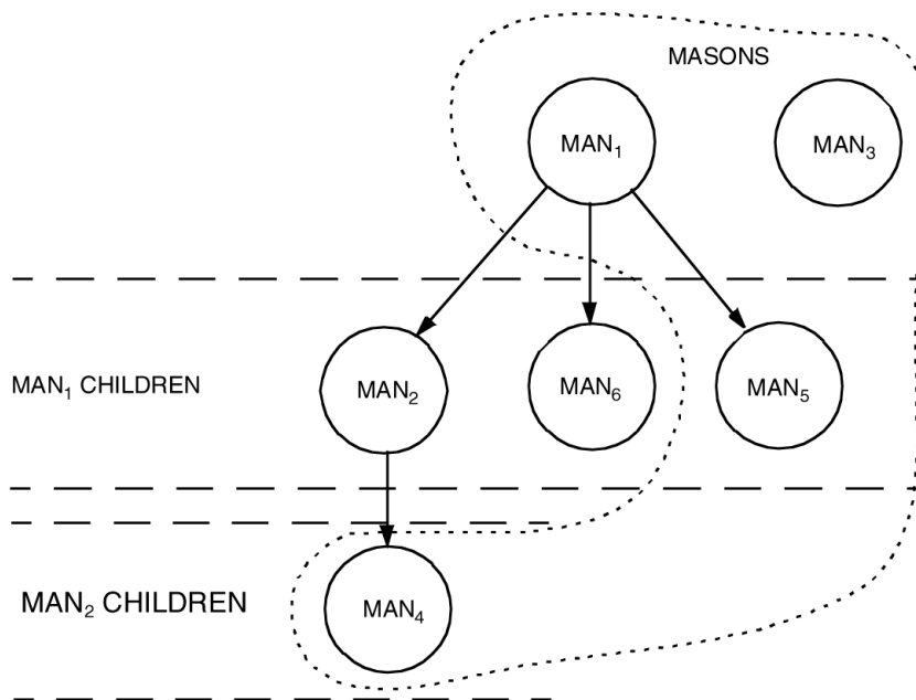
Figure 4-7. Set Relationships
