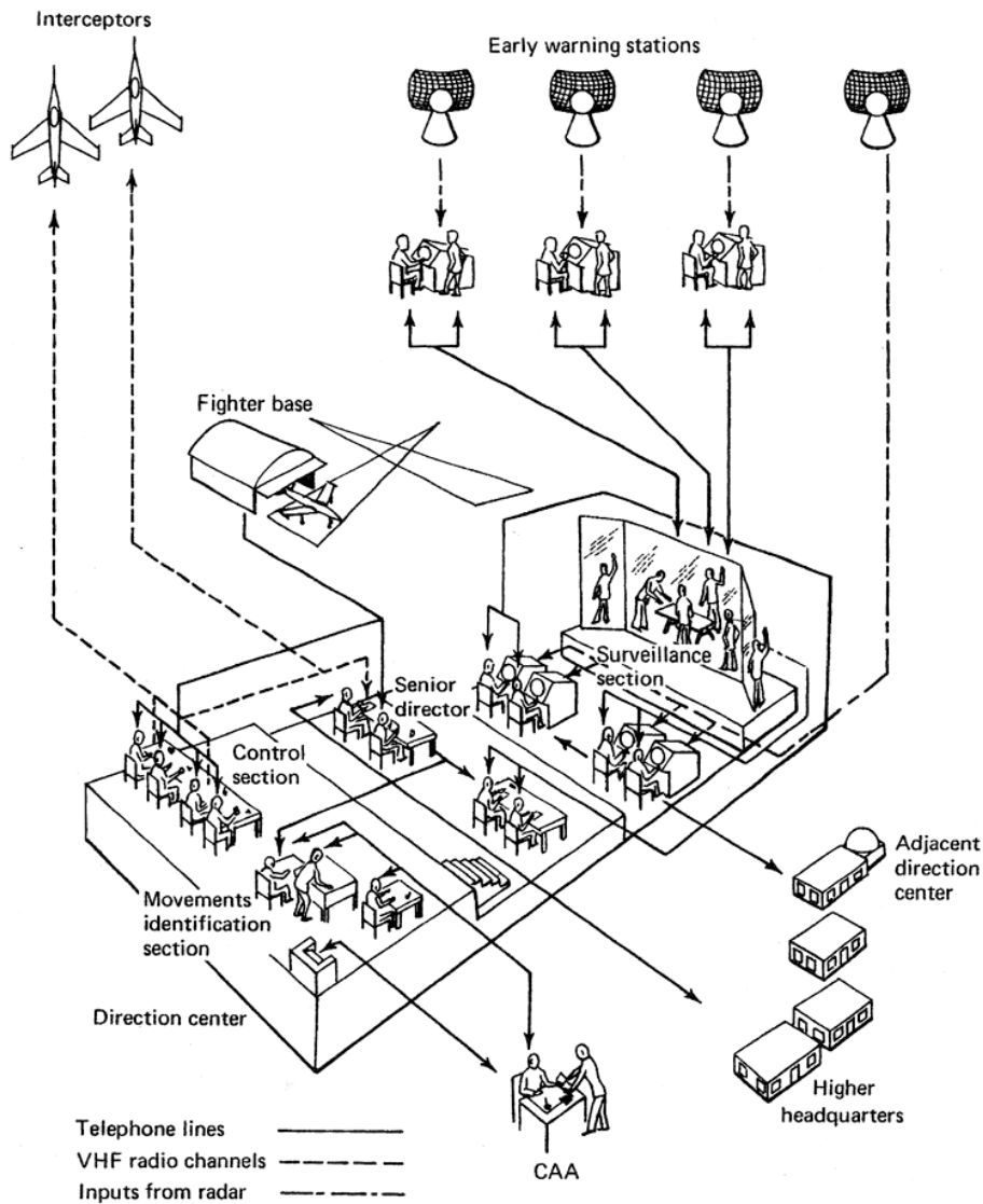
FIG. 9-2. Simplified model of Direction Center, RAND's System Research Laboratory Air Defense Simulation setup. This simplified model emphasizes aspects of the direction center's operation not readily seen in the previous schematic of functions: the physical arrangements within the center and the complex communication net (consisting of telephone lines, VHF radio channels, and radar inputs) that linked crew members to each other and to the external embedding organizations. Much of the communication within the center itself is either visual or by face-to-face conversations. (From RAND paper by R. L. Chapman et al. Also published in Management Science , 5:255. Used with permission of the RAND Corporation.)
