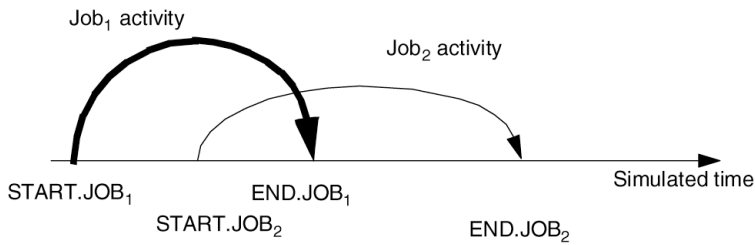
Figure 5-3a. Two Overlapping Activities
