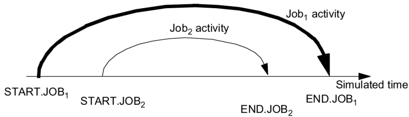
Figure 5-3b. Two Nested Activities
