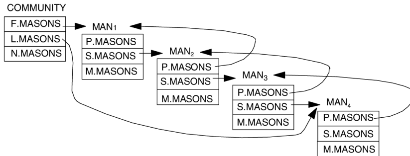
Figure 4-5. Owner-member Set Relationships
