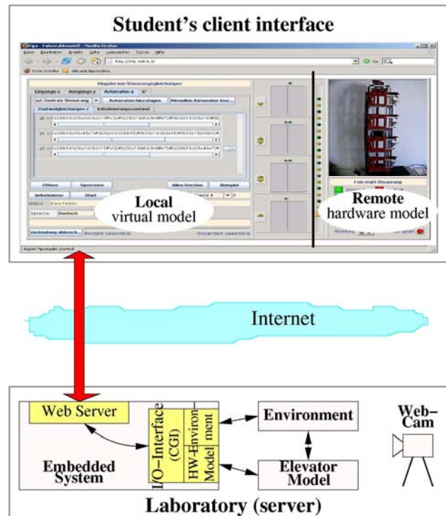
FIGURE 7: THE CLIENT-SERVER-ARCHITECTURE OF THE REMOTE LAB
