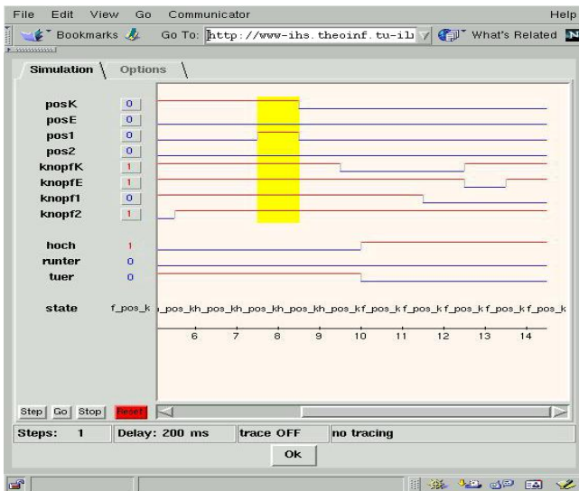
FIGURE 6: WAVEFORM SIMULATION FOR THE AUTOMATON "BEWEGUNG"
